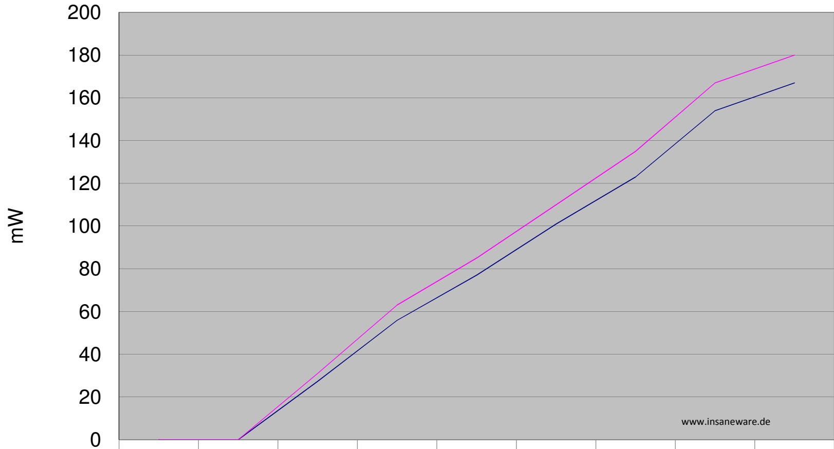
Laserbee I vs Coherent Lasercheck DPSS 532nm >150mW analog
